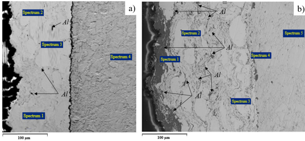
Figure 4. SEM-cross-sectional image of homogeneous (a) and gradient coating (b) based on Ni-Cr-Al.
