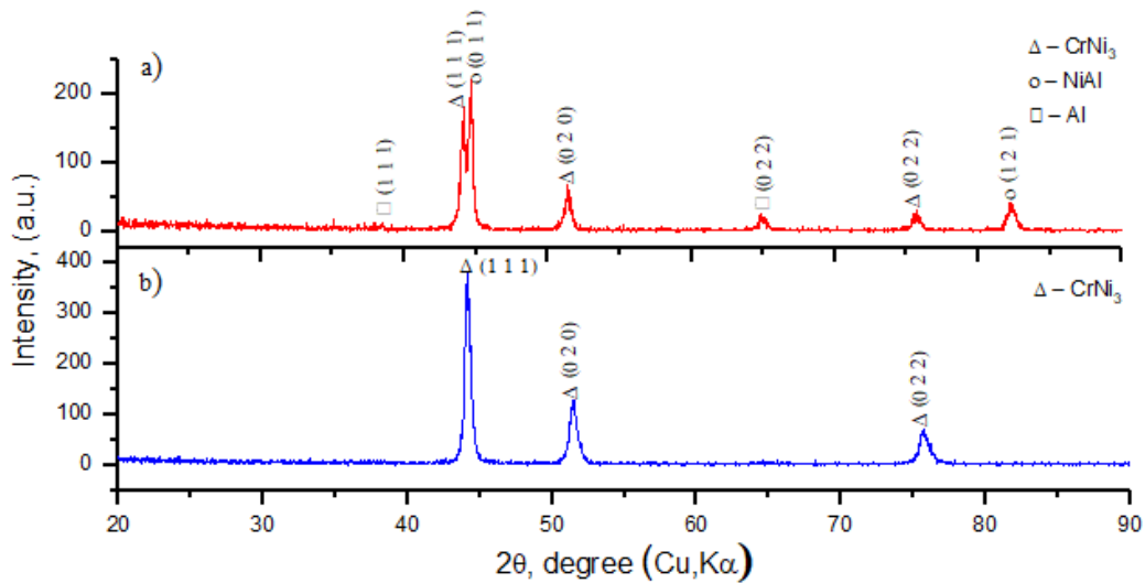
Figure 2. Diffractograms of single-layer and gradient coatings Ni-Cr-Al.
