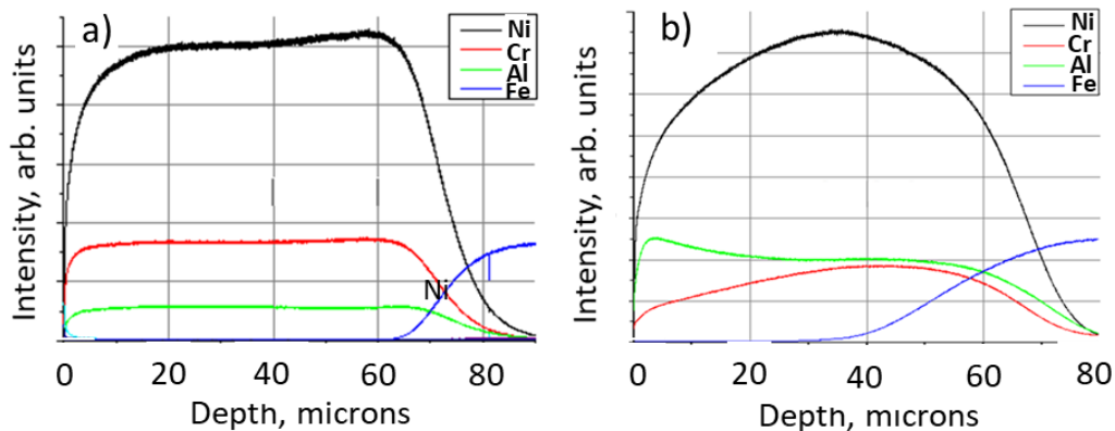
Figure 3. Depth distribution of elements of homogeneous (a) and gradient coatings (b) based on Ni-Cr-Al.
