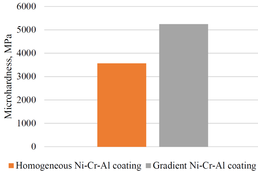
Figure 5. The results of microhardness of homogeneous and gradient Ni-Cr-Al coatings.
