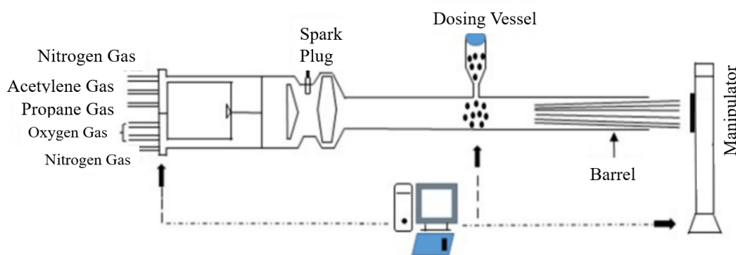
Figure 1. Computerized detonation complex CCDS2000: general view (a) and schematic diagram of the installation (b).
