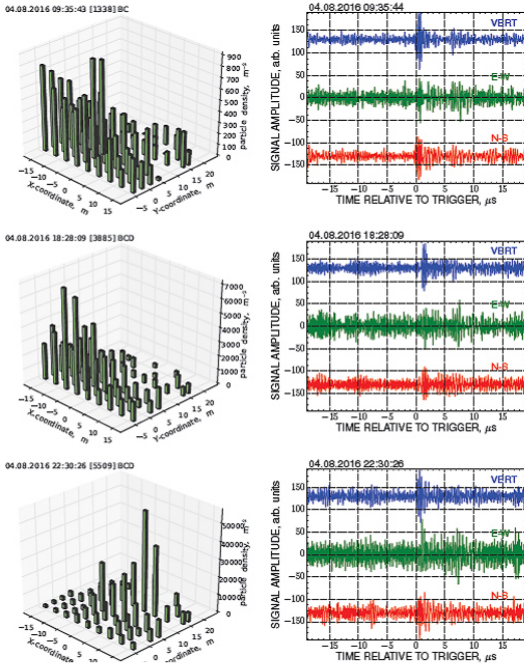
Figure 3. Sample events with a noticeable radio-signal from EAS. Left panels: 2D distribution of the density of charged shower particles in the plane of the central scintillation carpet; right panels: time series of the detected radio-signal amplitude from the vertical and two horizontal (East-West and North-South) antennae dipoles of the A1 point. Zero point of time axis in the right panel plots corresponds to the arrival time of the shower trigger.
