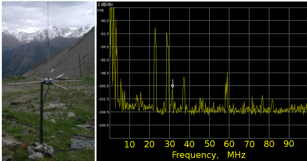
Figure 2. Three dipole antennae set installed at point A1 at the Tien Shan mountain station (left), and the spectrum of background radio-emission measured with the Agilent Technologies N1996A wave analyzer (right).
