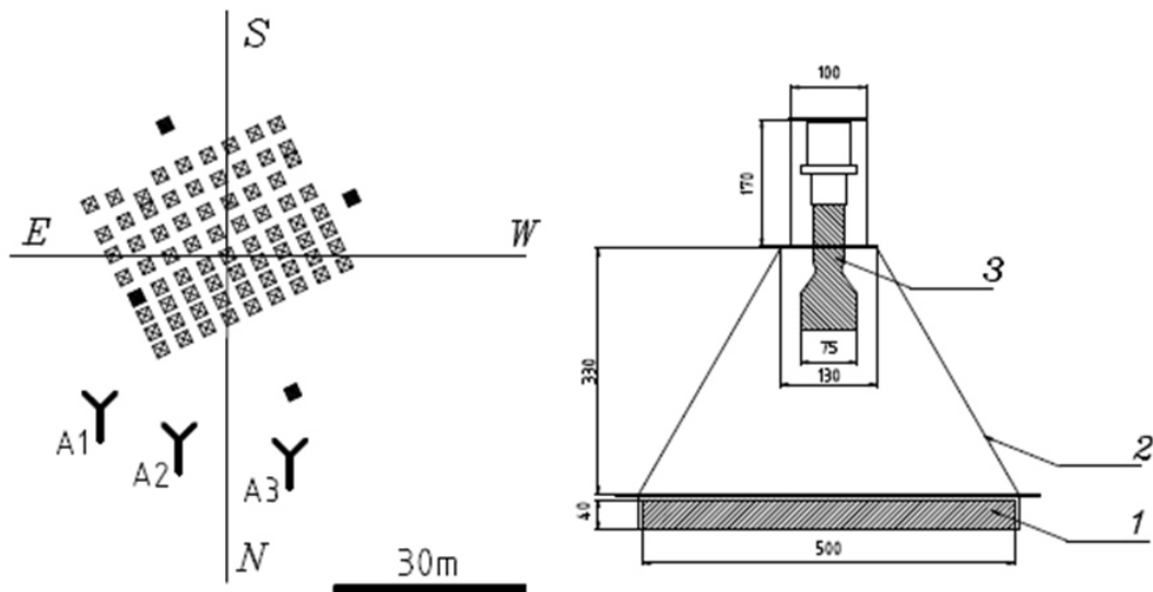
Figure 1. Left: the particle detector disposition scheme in the center part of the Tien Shan shower installation. Squares - the scintillation detectors of the central carpet, A1 - A3-the positions of the radio-antennae. Right: the internal arrangement of a scintillation detector (1 - a 500 \times 500 \times 40 \text{ mm}^3 plastic scintillator, 2 - the pyramid-shaped reflector of scintillation light, 3 - PMT; dimensions are shown in mm).
