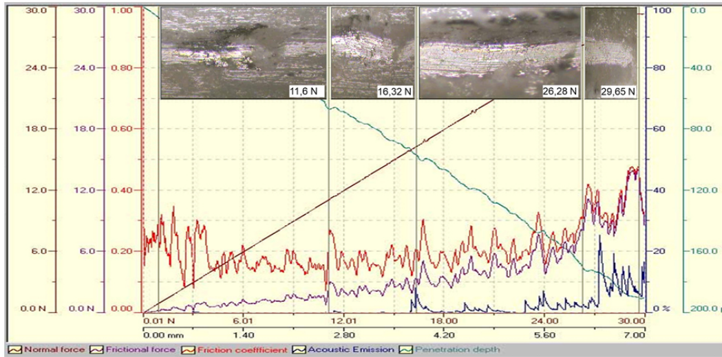
Figure 2. Results of the scratch test coatings made of zirconium dioxide.
