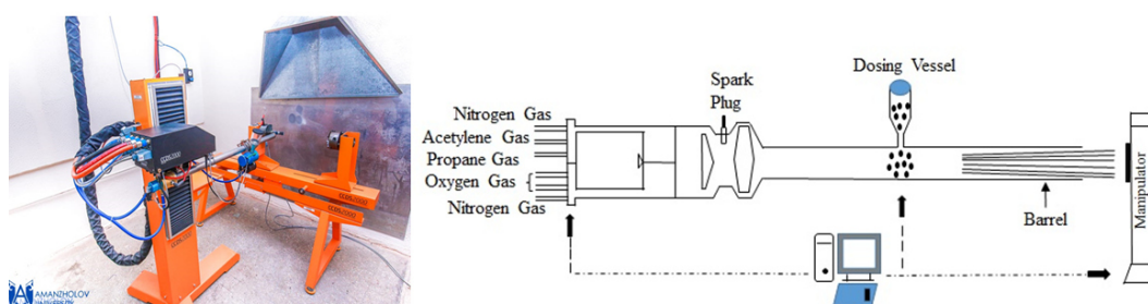
Figure 1. Computerized detonation complex CCDS2000 (a) and its circuit diagram (b).
