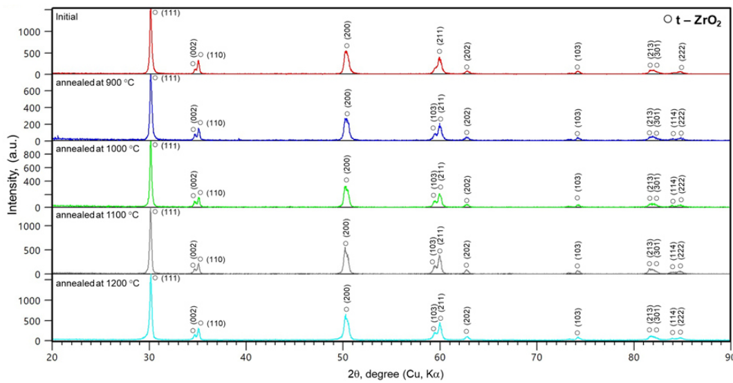
Figure 4. X-ray diffraction patterns of coatings from zirconium dioxide before and after annealing.
