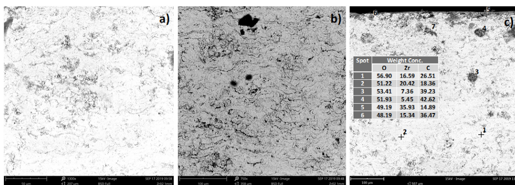
Figure 6. SEM-image of the surface (a), cross-section (b) of coatings of zirconium dioxide and the results of micro X-ray spectral analysis (c).
