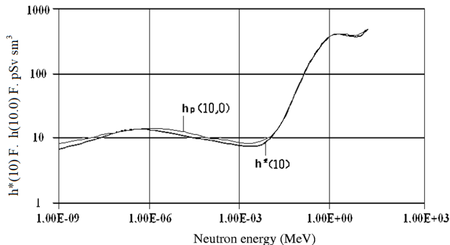
Figure 1. The energy dependence of specific individual ( h_p(10) ) and ambient dose ( h^*(10) ) equivalents.
