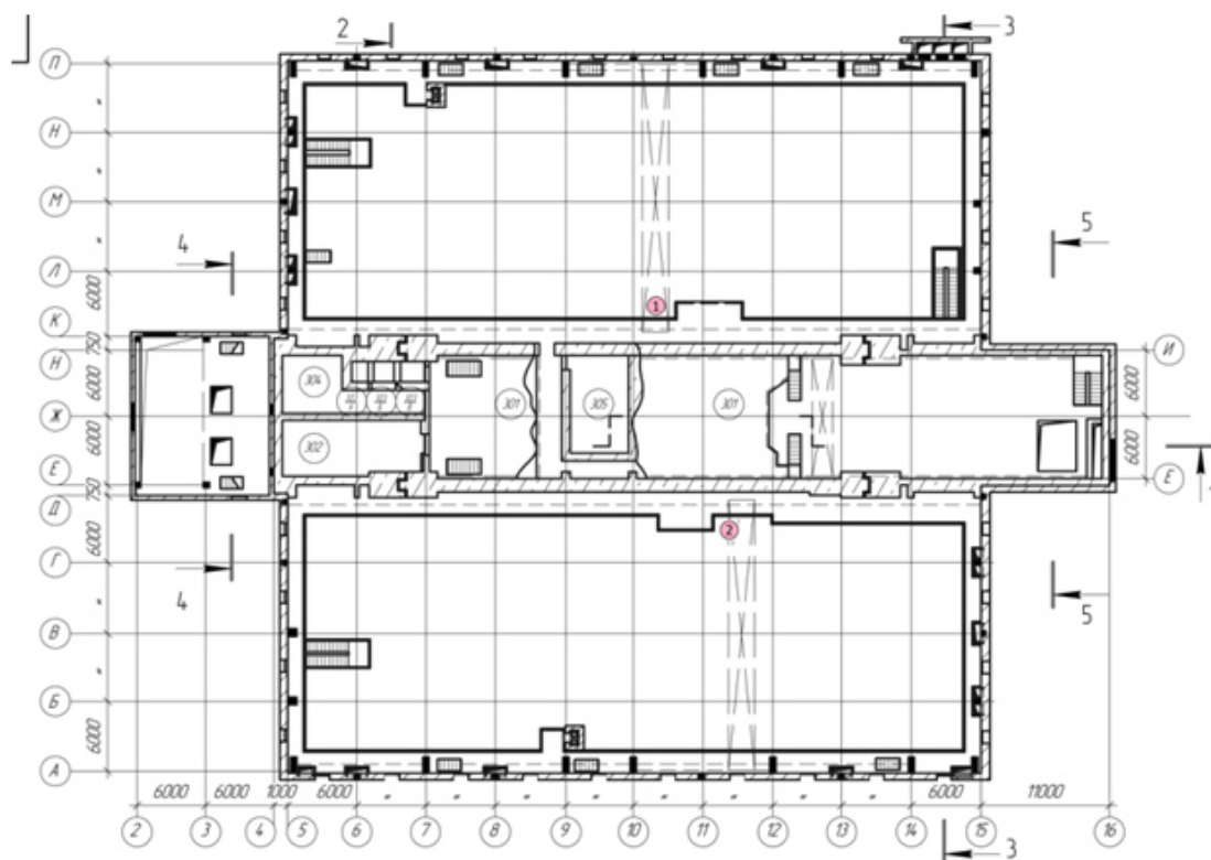
Figure 3. Plan of the IBR-2M experimental halls and measurement points.
