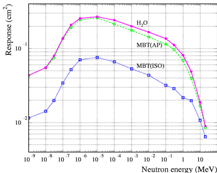
Figure 2. EDR of the albedo dosimeter DVG-01: H 2 O – water phantom in the form of a parallelepiped with dimensions of (30x30x15) cm with plexiglass sides; MBT(AP), MBT(ISO) – tissue equivalent (MBT – soft biological tissue) elliptic cylinder with dimensions of (20 × 40 × 60) cm.
