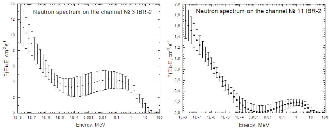
Figure 5. Spectra of neutrons at points 1 and 2. The average energy of the spectrum at point 1 is 218 keV, at point 2 it is 129 keV.
